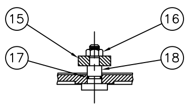
SECTION A-A FOR HANDWHEEL OPERATORS POSITION INDICATOR
