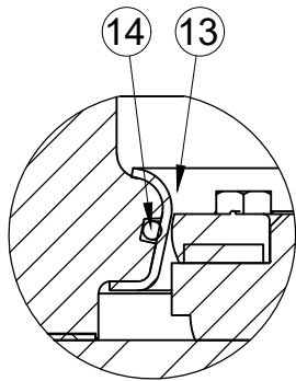
SEAT DETAIL
